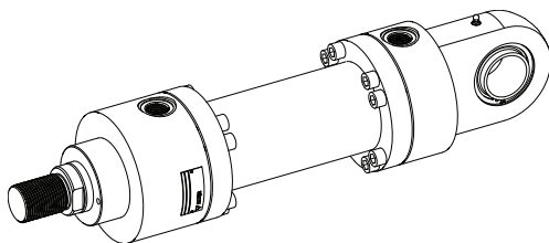
S (ISO MP6) = fixed eye with spherical bearing mounting
